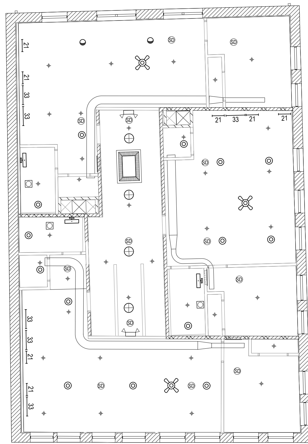
REFLECTED CEILING PLAN
